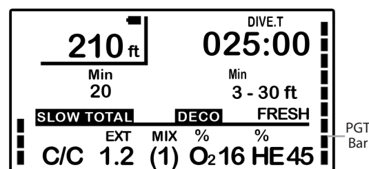
Primary Underwater Screen Decompression Symbol
